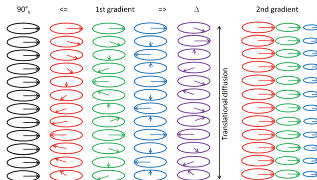
Fig. 2 A standard, 90^\circ_x pulse aligns the magnetization in the x-direction of the x–y plane (black arrows). The 1st gradient pulse (encode) twists this magnetization along in the x–y plane and along the z-axis into a corkscrew shape. The degree of the corkscrew effect depends on the strength of the gradient pulse (2%, red; 50%, green; 95%, blue). Samples diffuse vertically during the (translational) diffusion time (big delta, \Delta ) between the two gradient pulses (purple) – the degree of mixing will be greater for higher gradient strengths. As a result, only part of the magnetization (smaller arrows/circles) are recovered by the 2nd, decoding pulse (colour coding matches the gradient strengths of the 1st gradient pulse). This means that higher gradients (green, blue) result in smaller circles/magnetization/detected signals.
